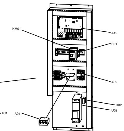
Electrical cabinet detailed view
