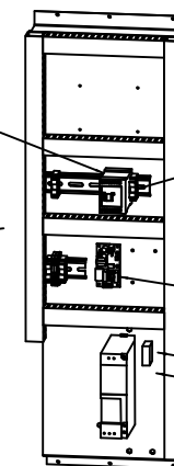
Electrical cabinet detailed view
