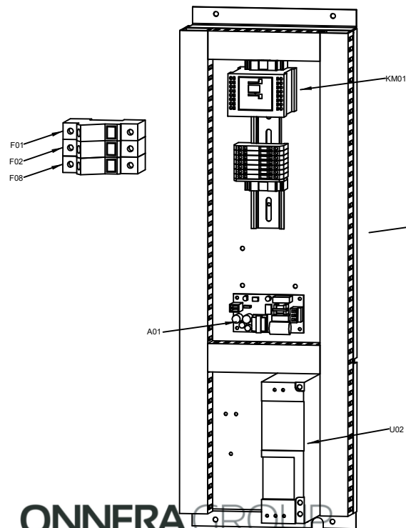
Electrical cabinet detailed view
