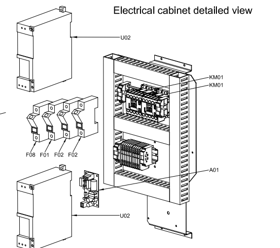
Electrical cabinet detailed view
