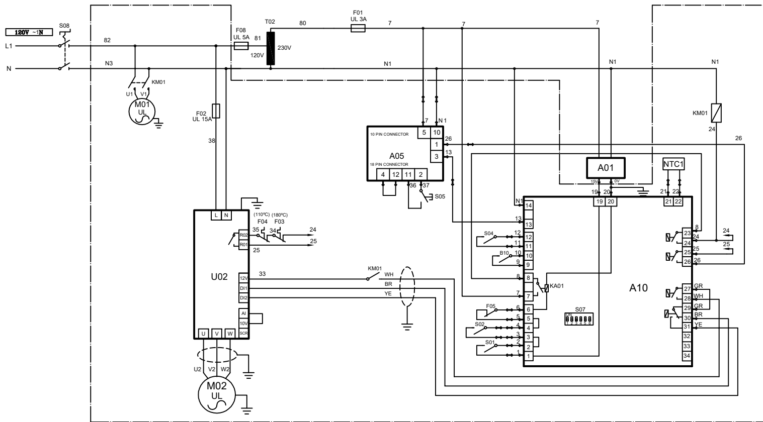
Electrical cabinet detailed view
