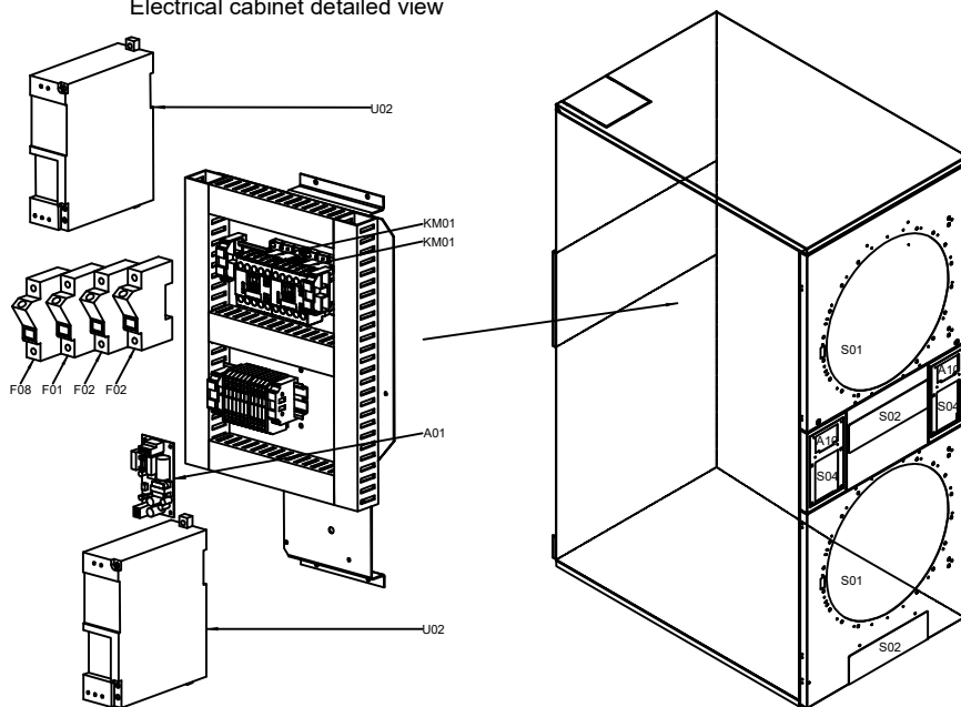
Electrical cabinet detailed view
