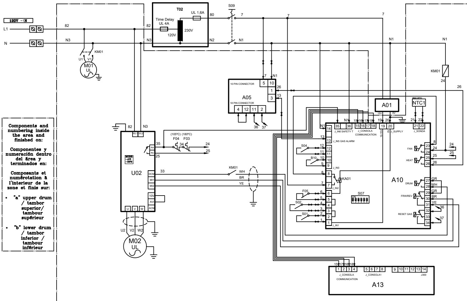
Electrical cabinet detailed view
